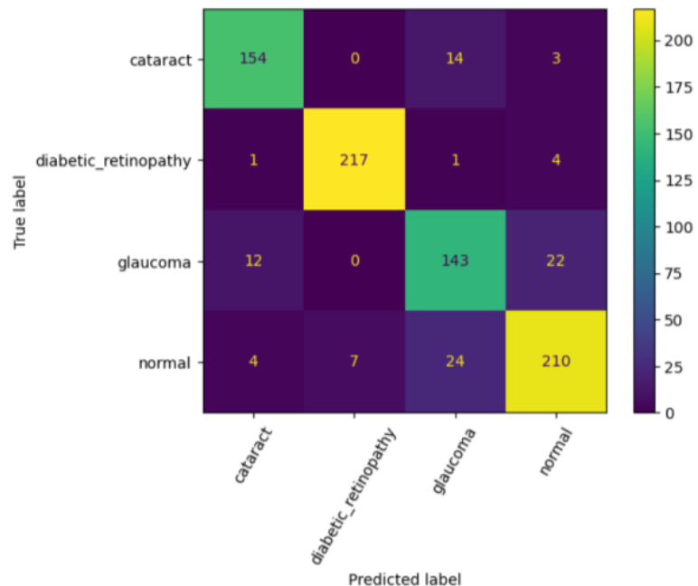
Test (Hold-out) Confusion Matrix highlighting the predictive skill of the Image Classification Model
